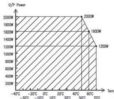
POWER DERATING CURVE (When 264VAC ≥ I/P > 180VAC)
