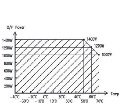
POWER DERATING CURVE (When 180VAC ≥ I/P > 90VAC)
