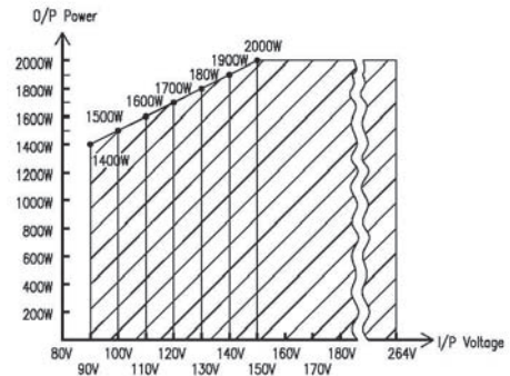
POWER DERATING CURVE (When T_a \leq 50^\circ\text{C} )
